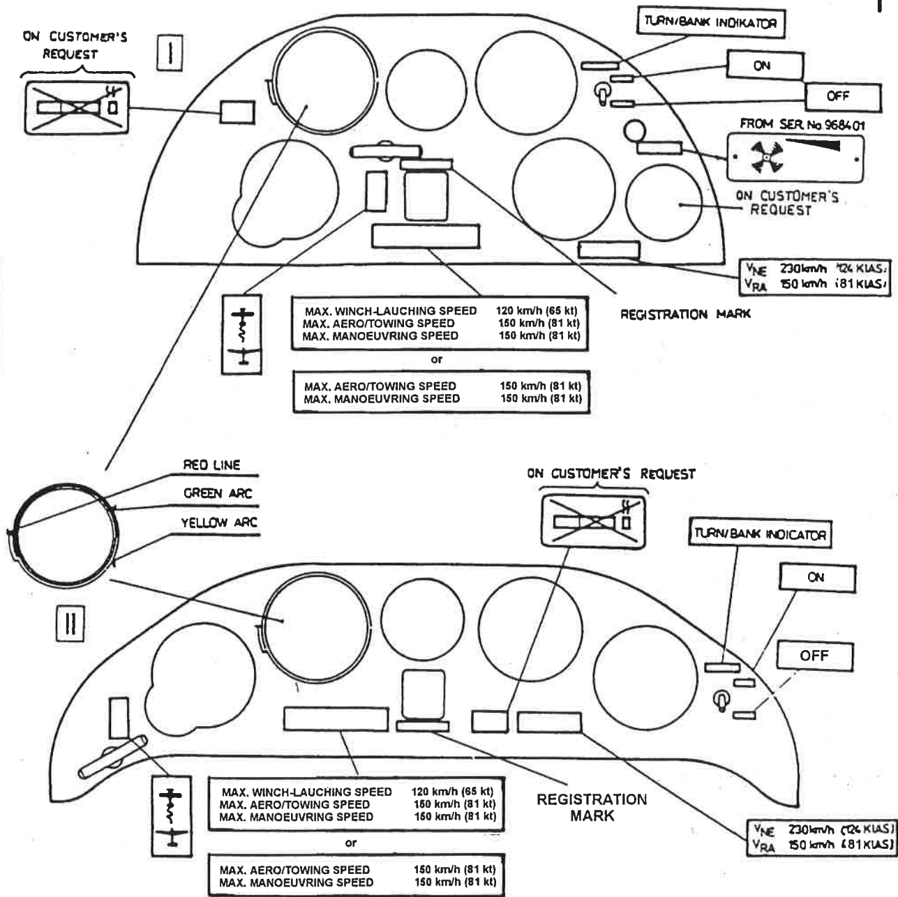
FIG. 3 INTERIOR PLACARDS AND MARKINGS IN THE SAILPLANE - FRONT AND REAR INSTRUMENT PANEL
